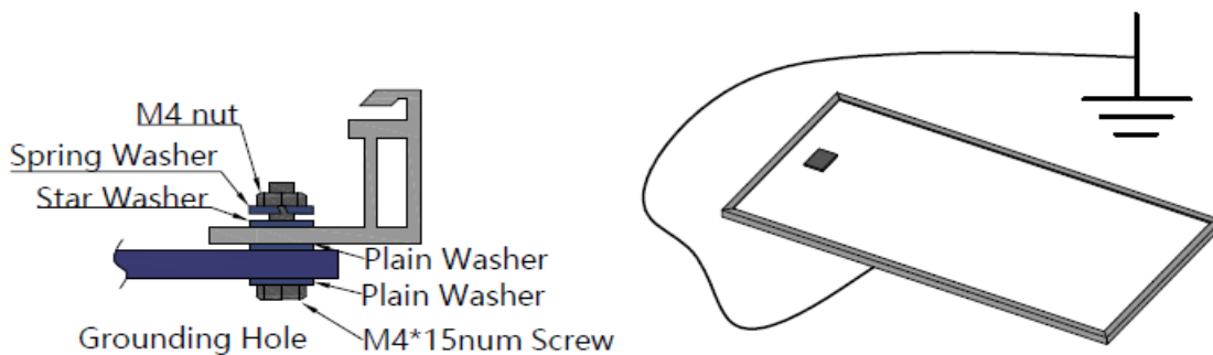
Figure 8: Ground installation of PV modules
