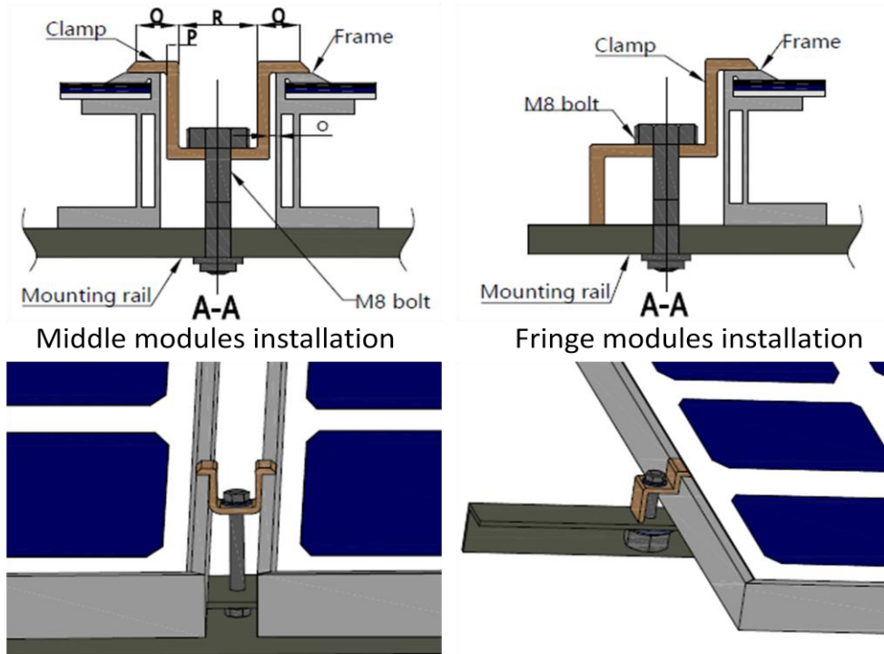
Figure 4: PV module installed at the side with Clamp fitting method
