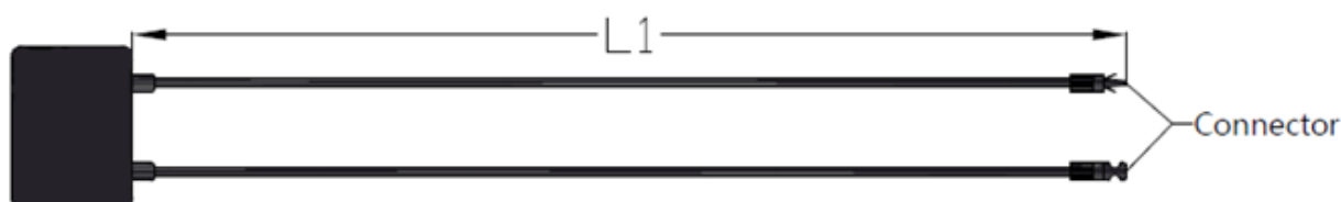
Figure 10: Junction box
